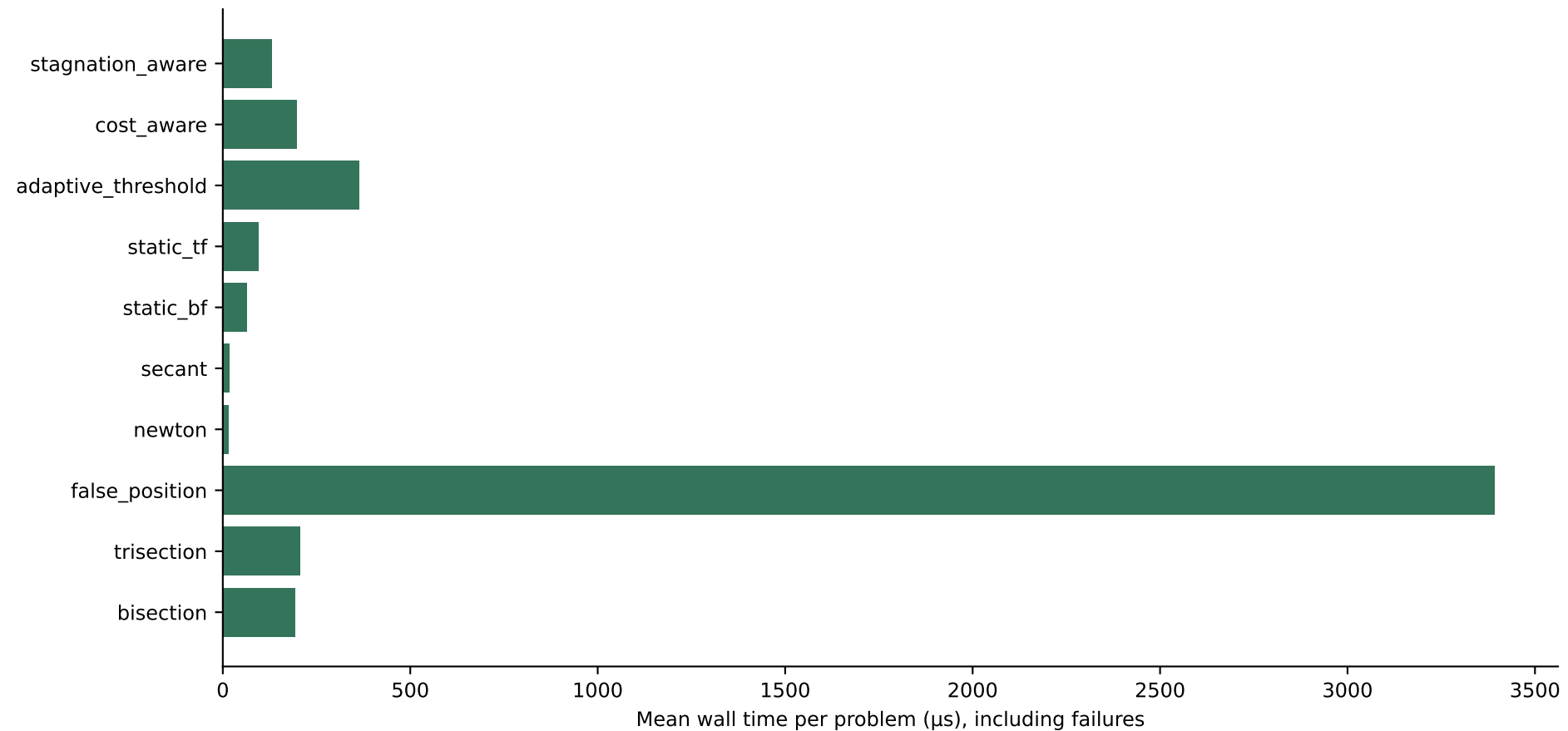
Stress benchmark — execution time
