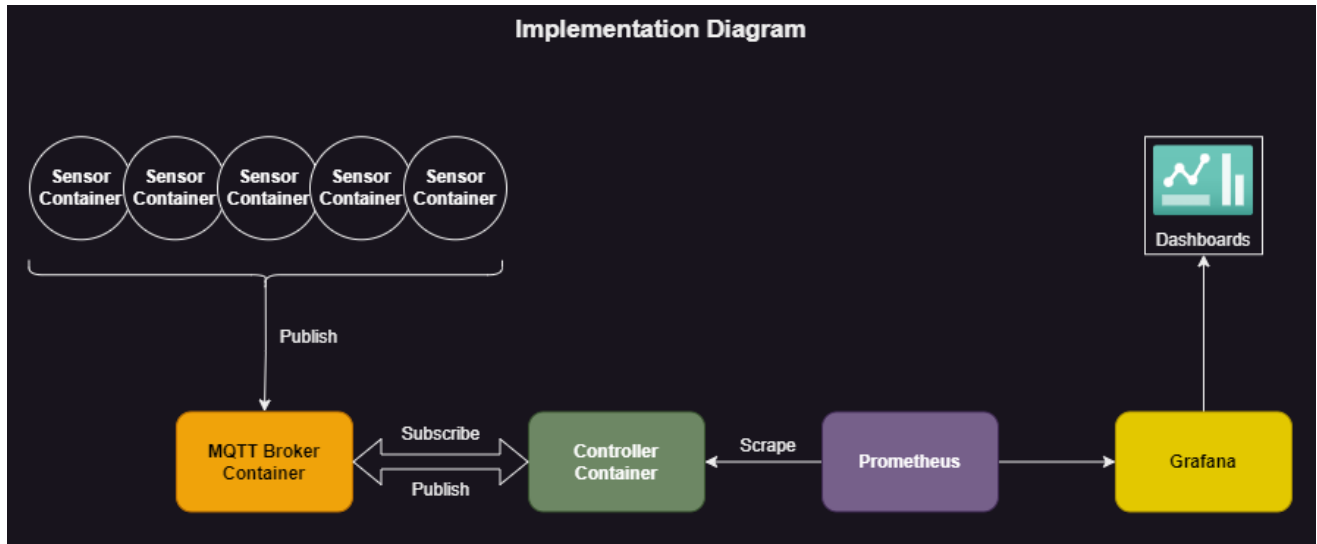
Figure 6.1: Implementation Diagram
