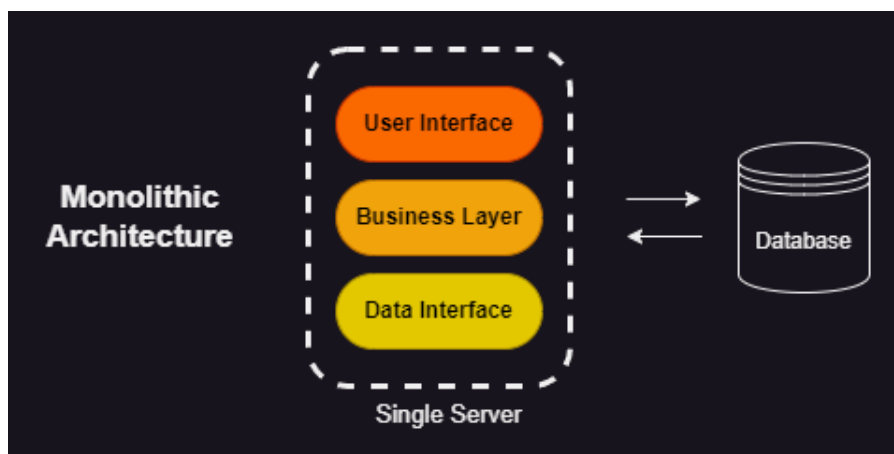
Figure 3.1: Monolithic Architecture
