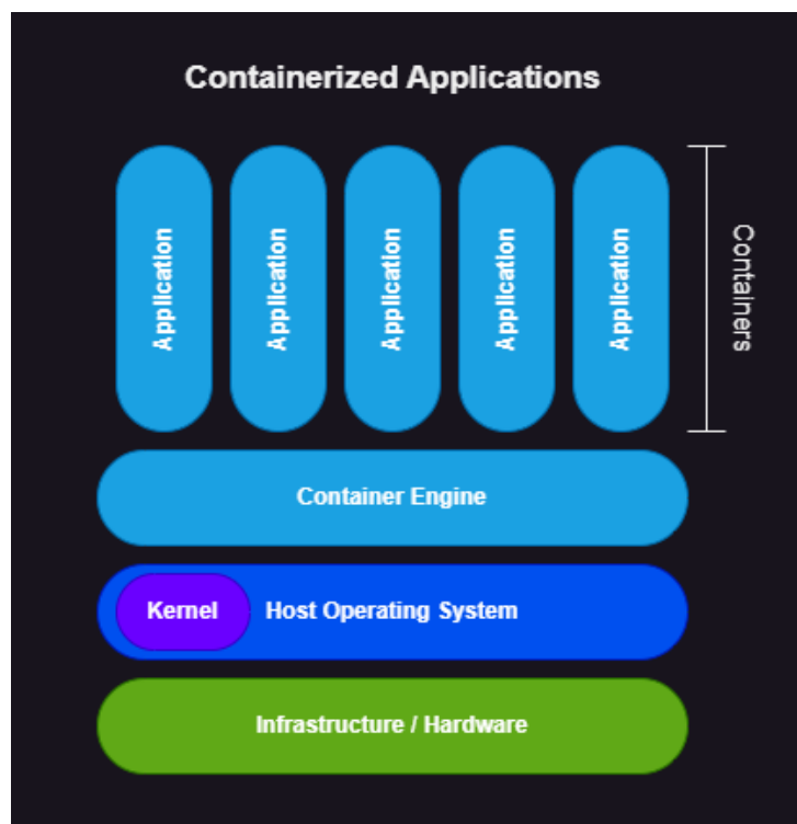
Figure 3.3: Containerized Applications
