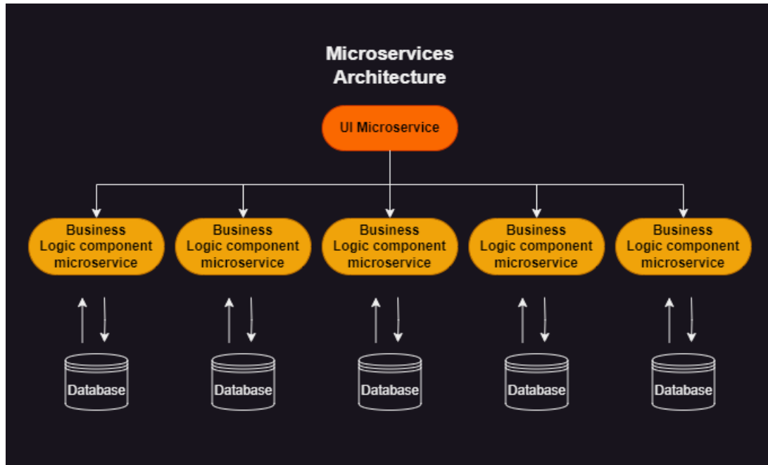
Figure 3.2: Microservice Architecture
