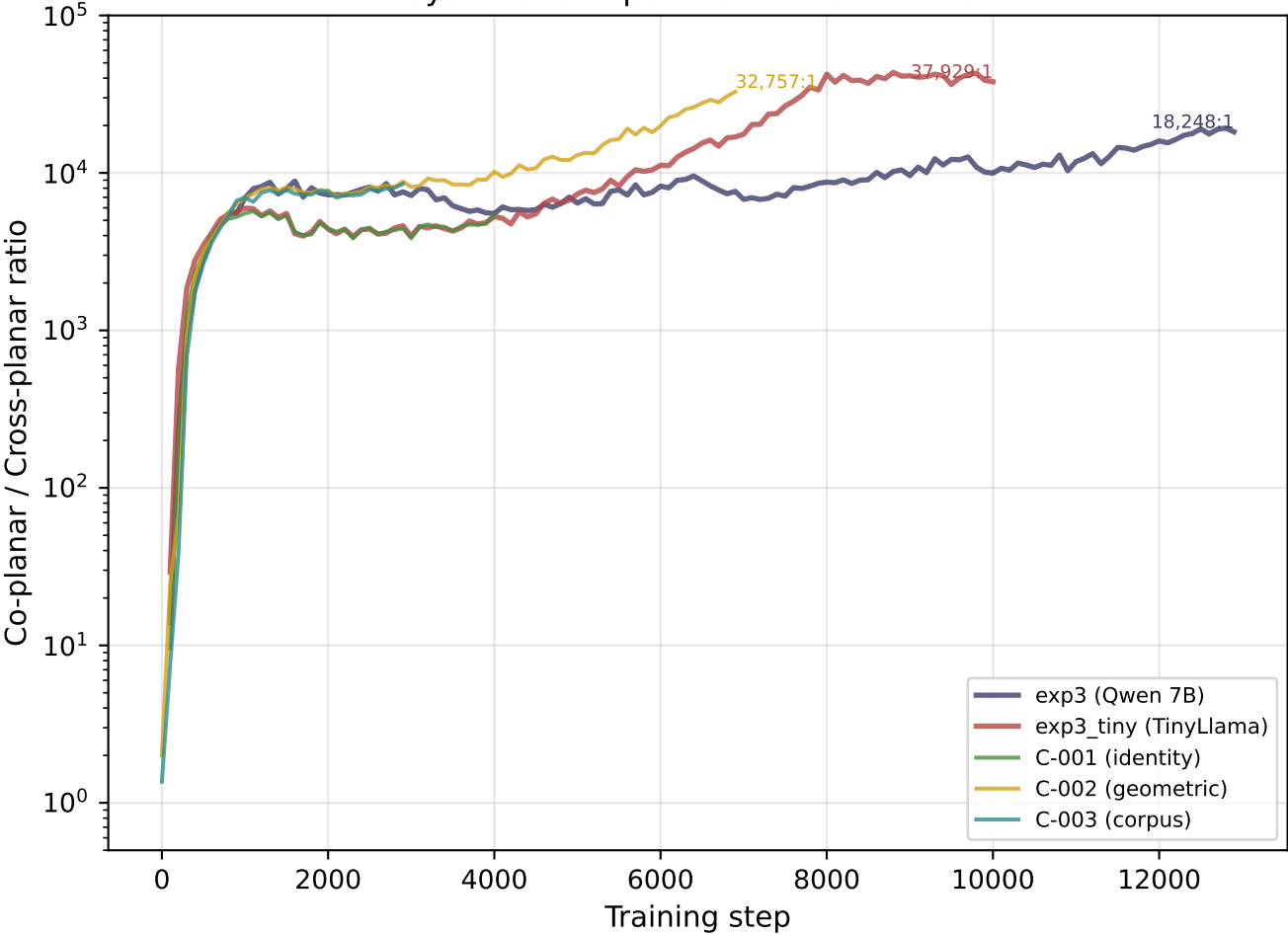
All Cybernetic Experiments: Ratio Evolution
