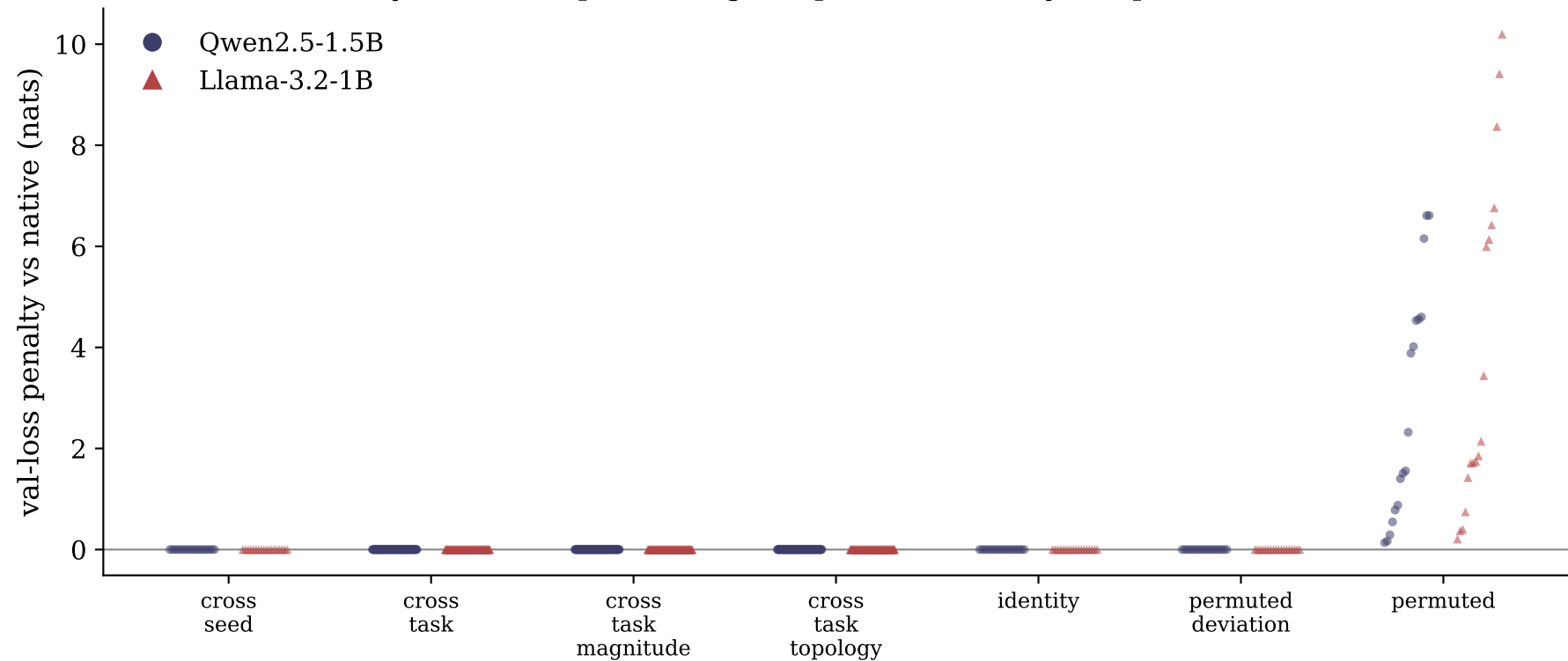
D2: every backbone-preserving swap costs \sim 0 ; only full permutation costs
