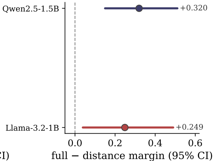
Margin: both CIs exclude 0
