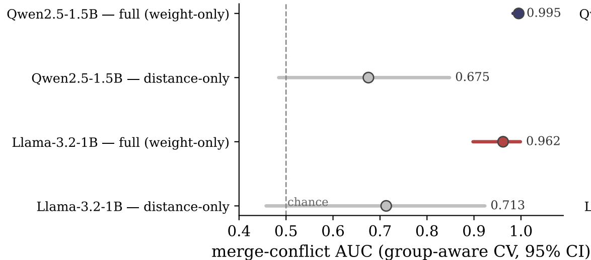
D3: weight-only features vs distance baseline
