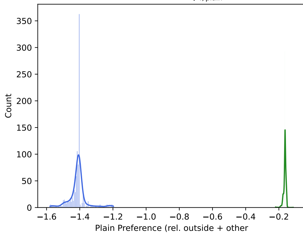
Distribution of \beta_{i, \text{plain}}
