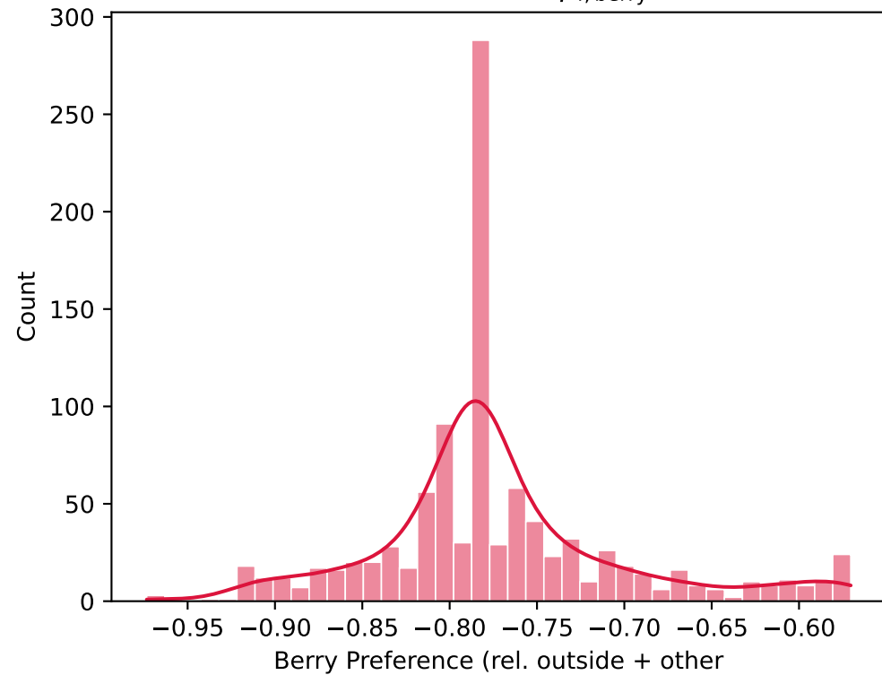
Distribution of \beta_{i, \text{berry}}
