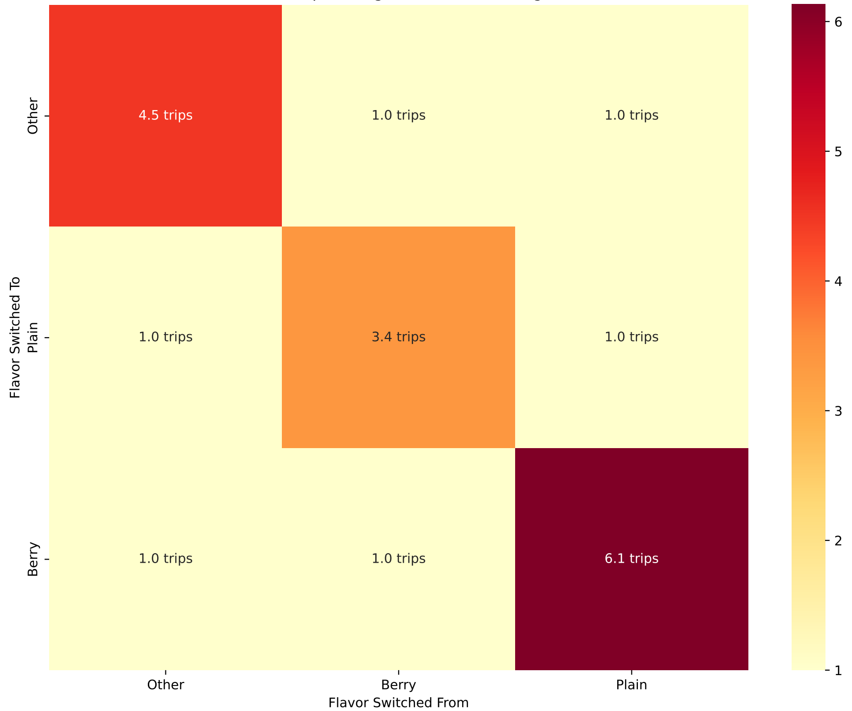
Mean Spell Length Prior to Switching
