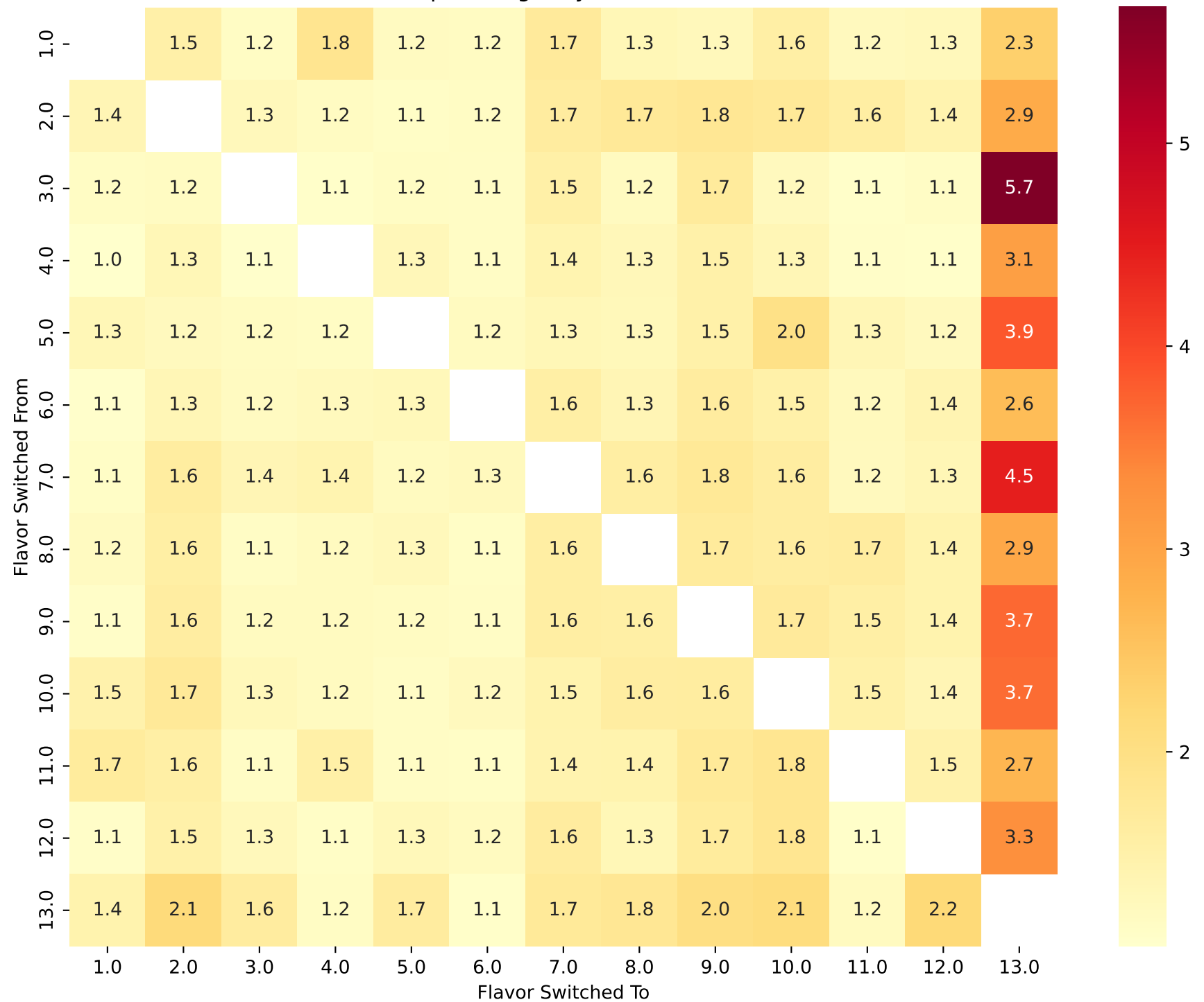
Mean Spell Length by Flavor Transition
