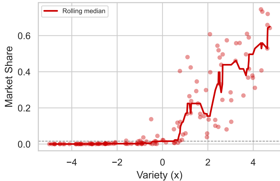
Target
