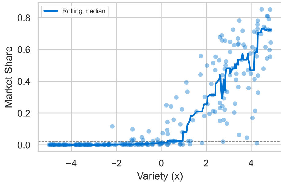
Walmart
