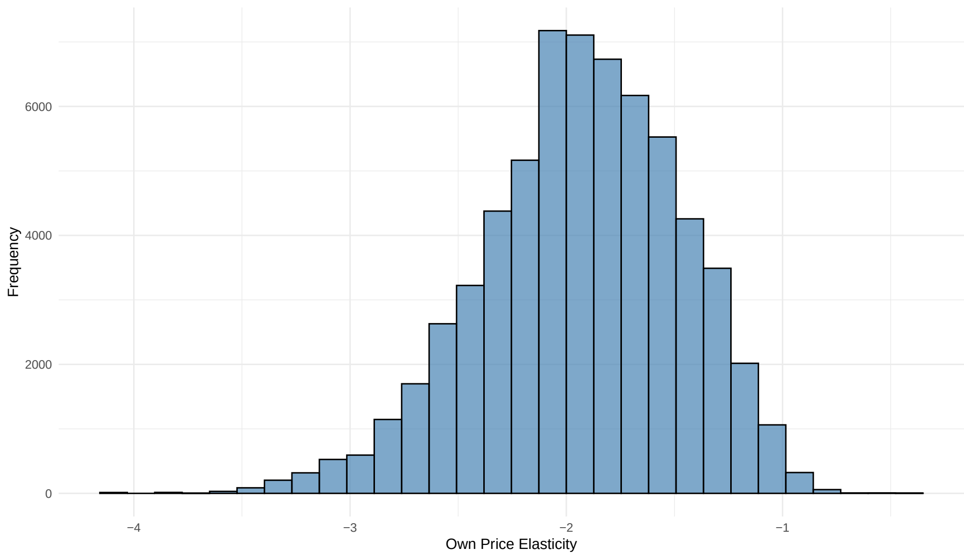
Histogram of Own Price Elasticities
