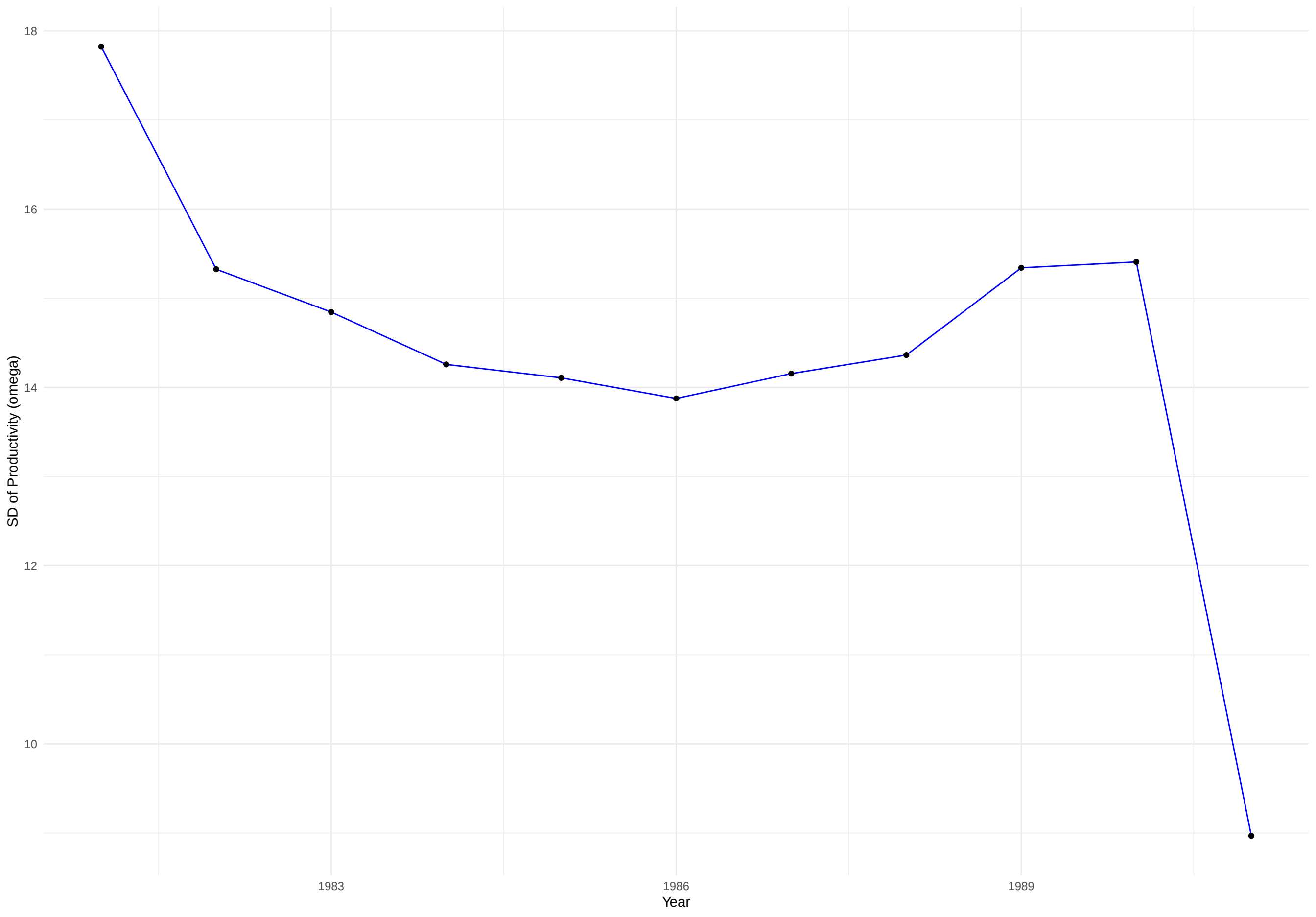
Standard Deviation of Productivity Over Time (Colombia)
