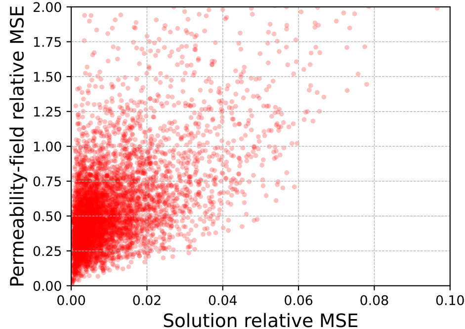
Test case 2: Prior
