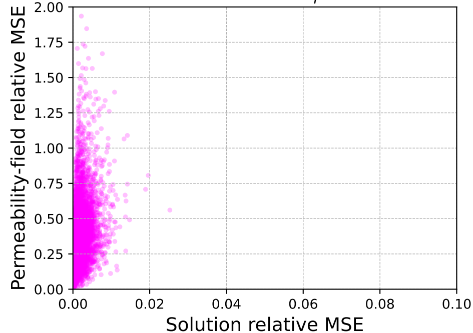
Test case 2: NN: \sigma_Y^2 = 10^{-6}
