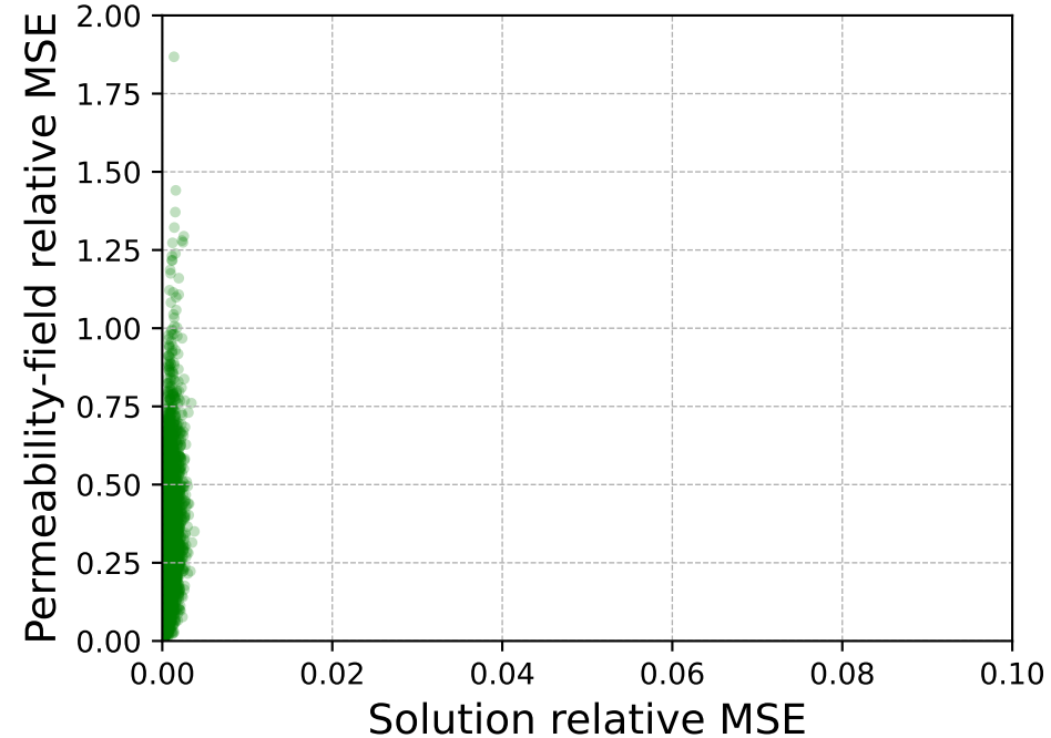
Test case 2: MCMC
