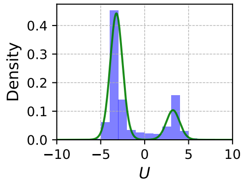
DM: y = -0.25 \cdot \mathbf{1}_{10}
