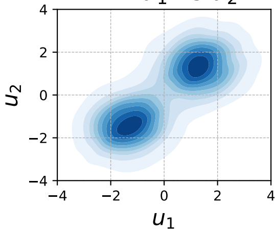
NN: u_1 vs u_2
