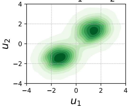
True: u_1 vs u_2
