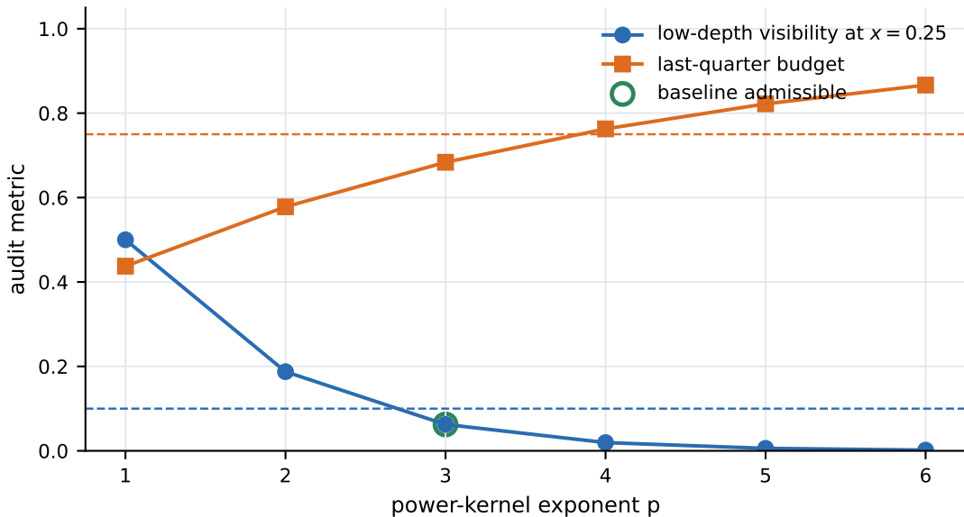
Shape-selection audit for simple power kernels
