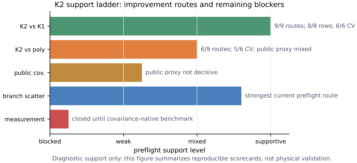
Figure 6: K2 support ladder. The figure summarizes reproducible improvement routes and blockers: K2 is consistently stronger than K1/no-memory at preflight level, conditionally supportive against flexible controls, and still blocked from measurement-validation language.
