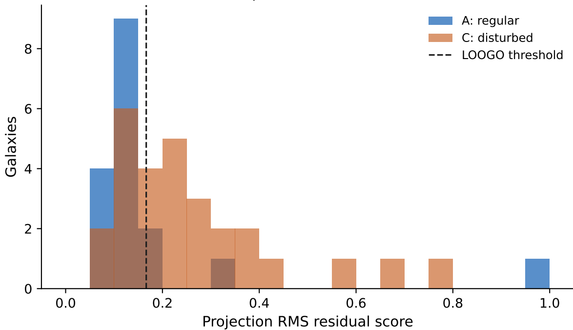
Residual-score separation of external A/C classes
