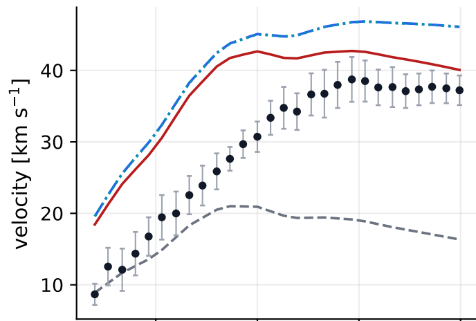
DDO126 rotation curve
