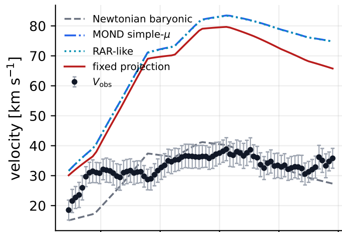
DDO50 rotation curve
