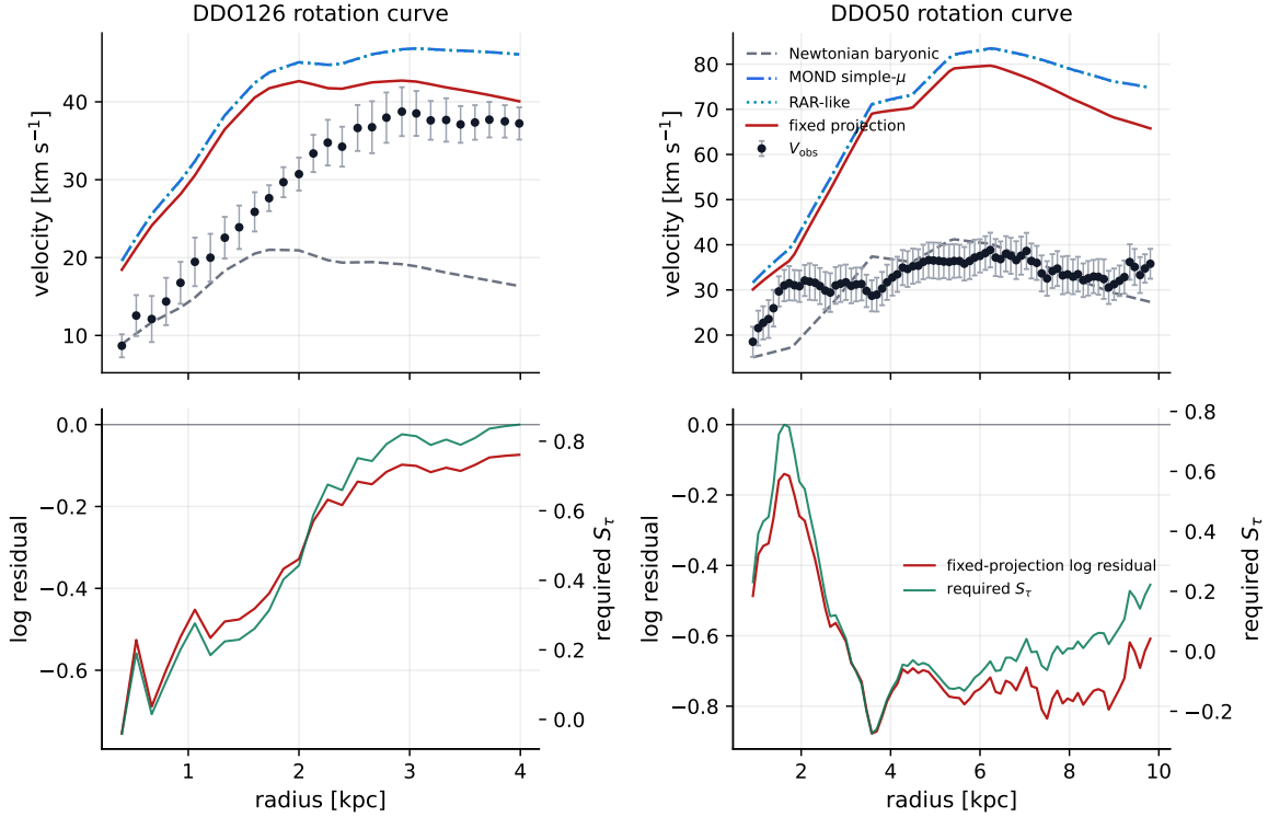
Figure 2: Illustrative rotation-curve diagnostics for DDO126 as a positive anchor and DDO50 as a control object. The panels show how the residual-score families appear in actual rotation-curve space. This visualization is not a primary endpoint and is not used to tune the classifier.
