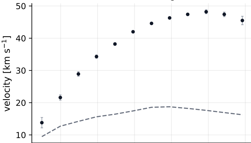
DDO154: correct regular A
