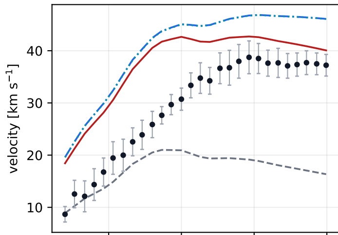
DDO126 rotation curve
