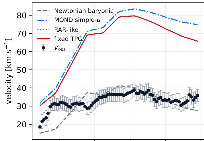
DDO50 rotation curve
