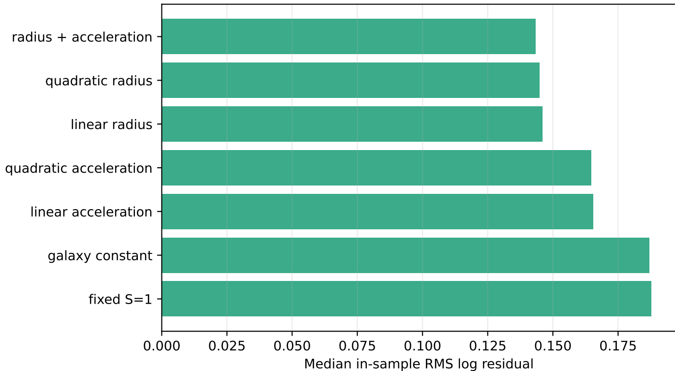
Required S_\tau function-family diagnostics
