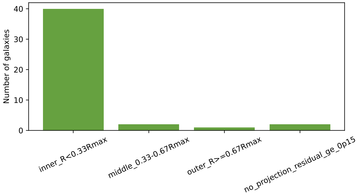
Where the TPG residual first exceeds 0.15 dex
