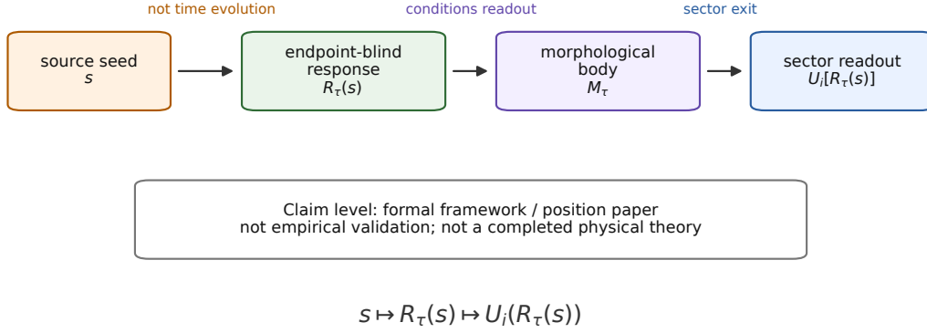
Figure 1: The minimal Tau Core spine used in Foundation Paper I. A parent-side seed s induces an endpoint-blind Tau response R_\tau(s) . A Tau-side morphological body M_\tau conditions sector readouts U_i . This is a formal architecture, not empirical validation.
