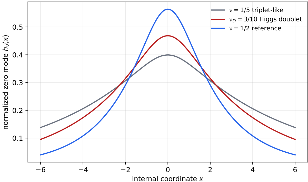
Tau-localized zero-mode profiles
