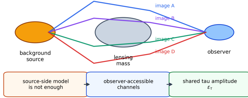
Figure 1: Schematic of the tau-core observer principle in a multiply imaged time-delay lens. The same background source reaches the observer through several image channels, making parity, Fermat structure, and time delays observer-accessible probes rather than source-only quantities.
