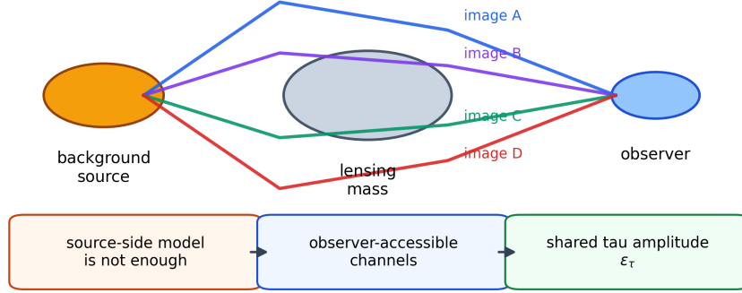
Figure 1: Figure 1. Schematic of the tau-core observer principle in a multiply imaged time-delay lens. The same background source reaches the observer through several image channels, making parity, Fermat structure, and time delays observer-accessible probes rather than source-only quantities.
