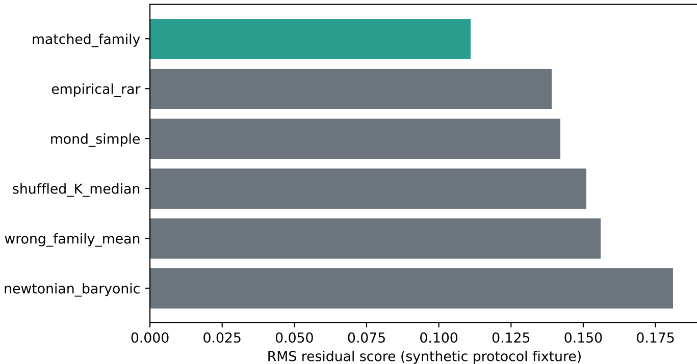
Forward gate endpoint: matched family versus controls
