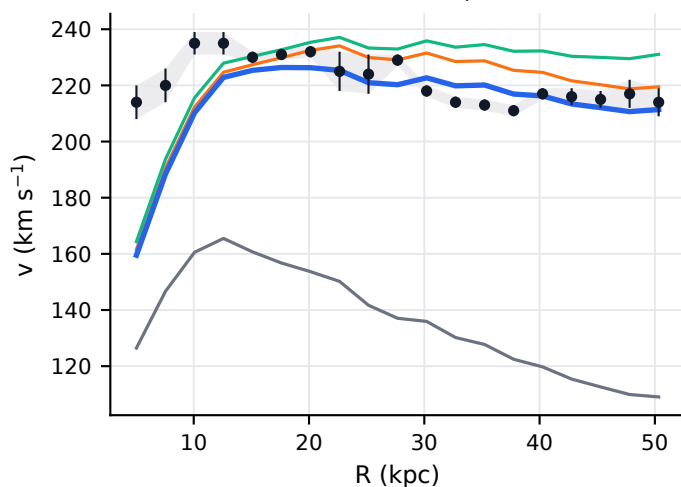
NGC4088: matched 11.6, baseline 25.4
