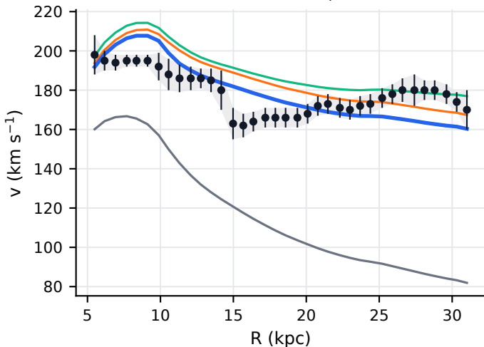
NGC7331: matched 22.3, baseline 23.5
