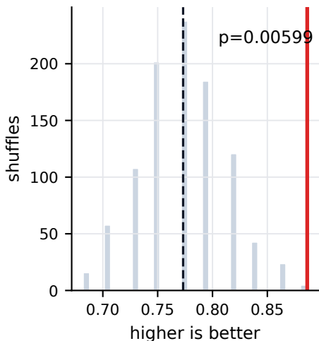
beats wrong-family fraction
