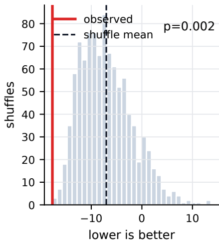
mean matched - wrong RMSE
