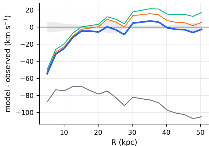
NGC4088: RMSE gain 13.8 km s -1
