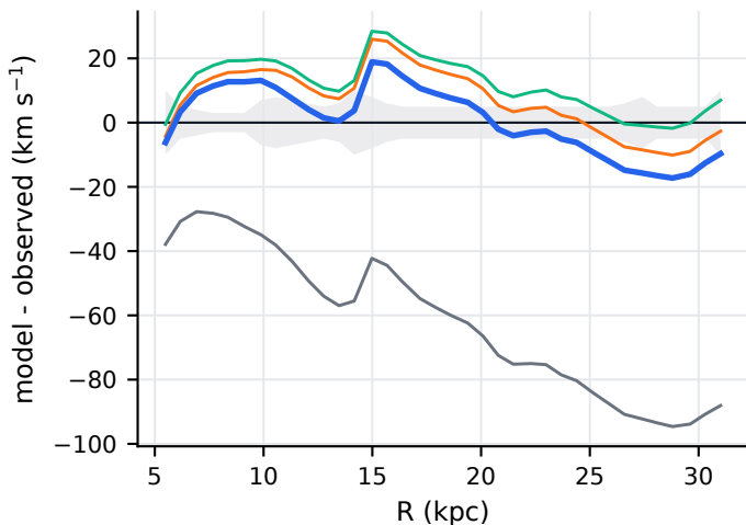
NGC7331: RMSE gain 1.2 km s -1
