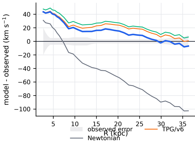
NGC7331: RMSE gain 1.2 km s -1
