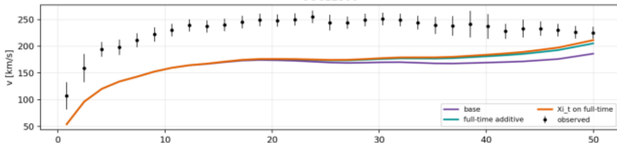
UGC12506
