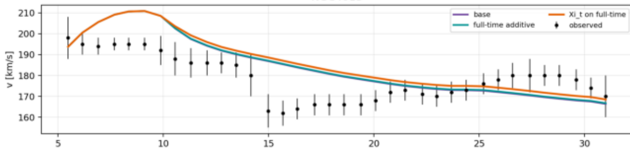
NGC4088
