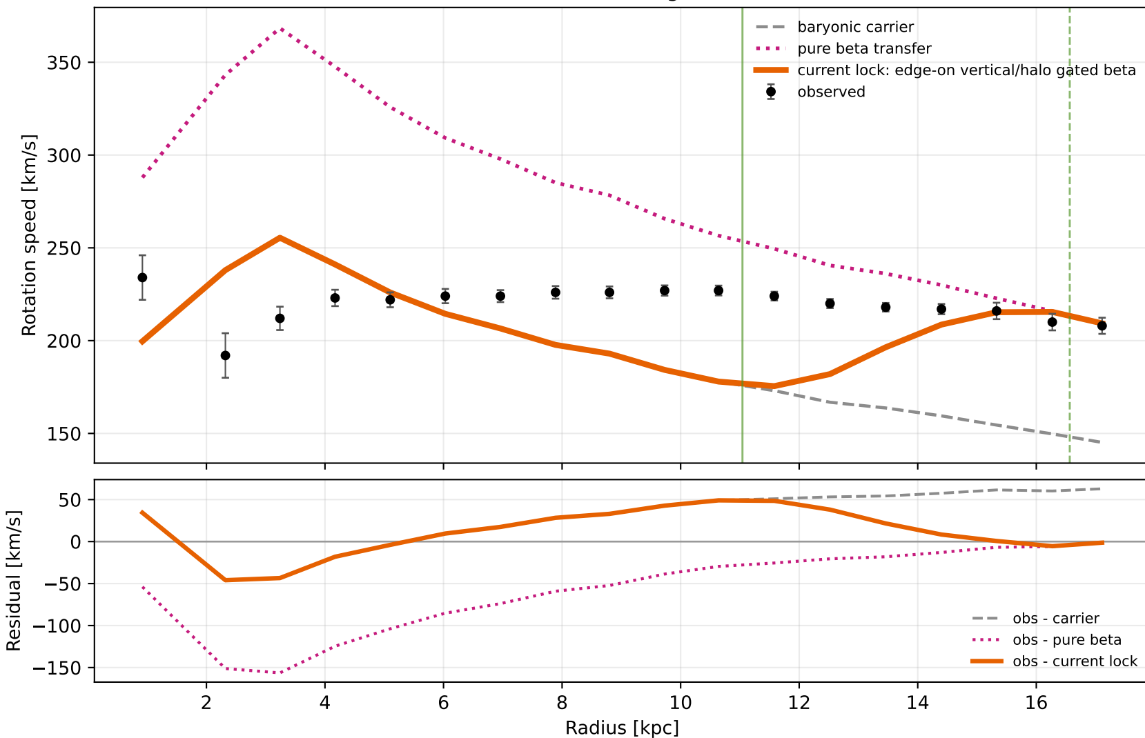
NGC0891: source-windowed edge-on vertical/halo lock
