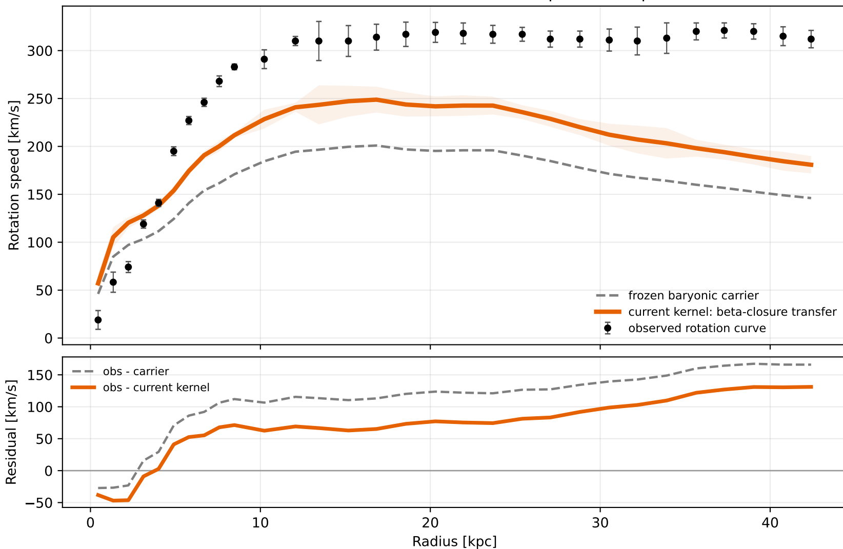
ESO563-G021: beta-closure transfer control comparison (improves carrier)
