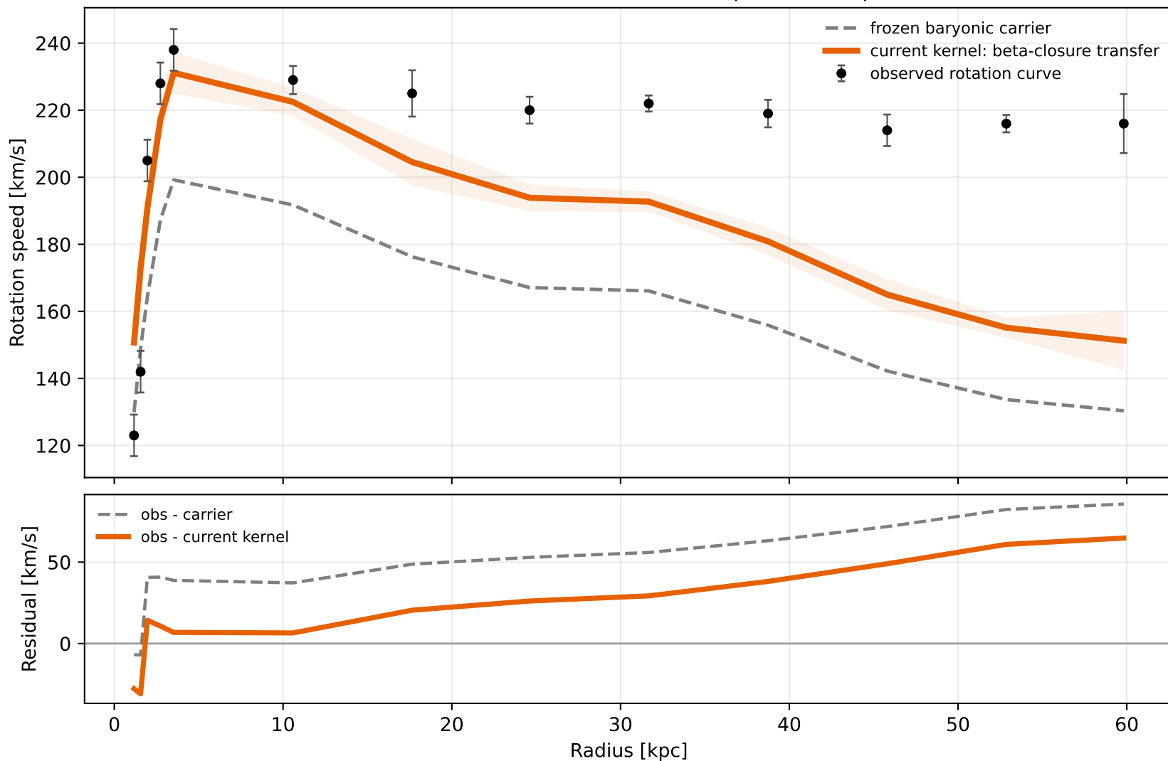
NGC0801: beta-closure transfer control comparison (improves carrier)
