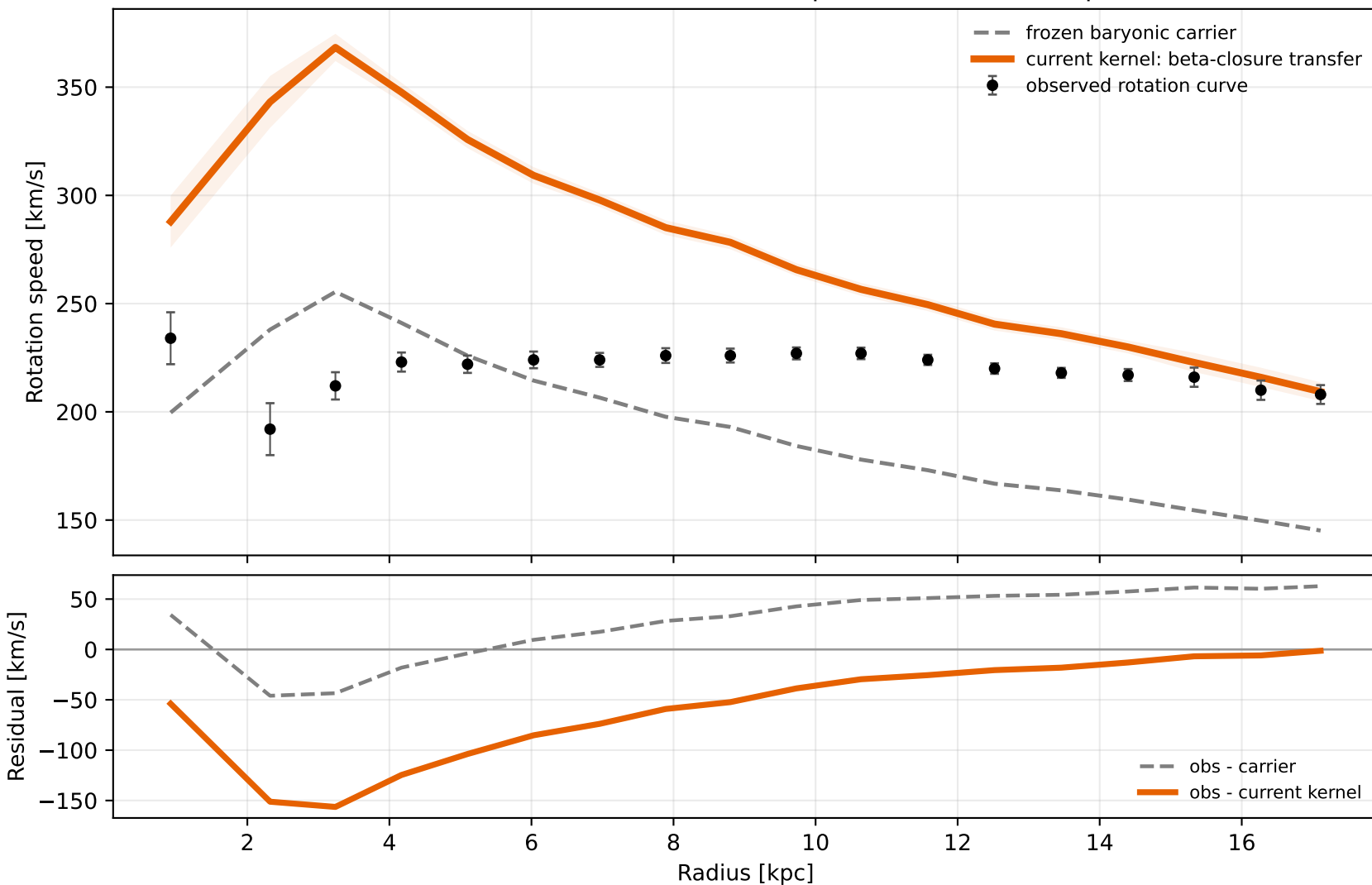
NGC0891: beta-closure transfer control comparison (does not improve carrier)
