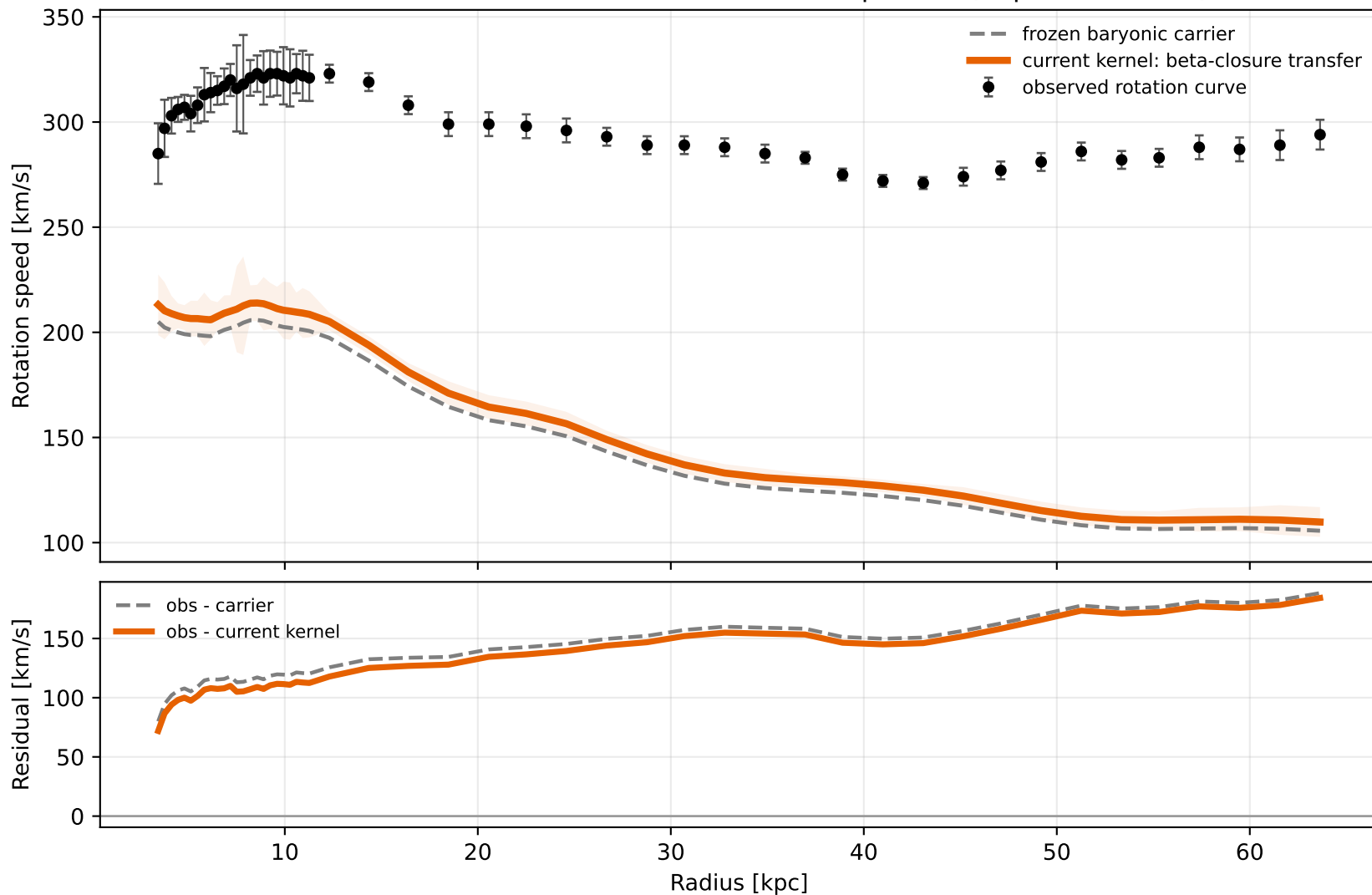
NGC2841: beta-closure transfer control comparison (improves carrier)
