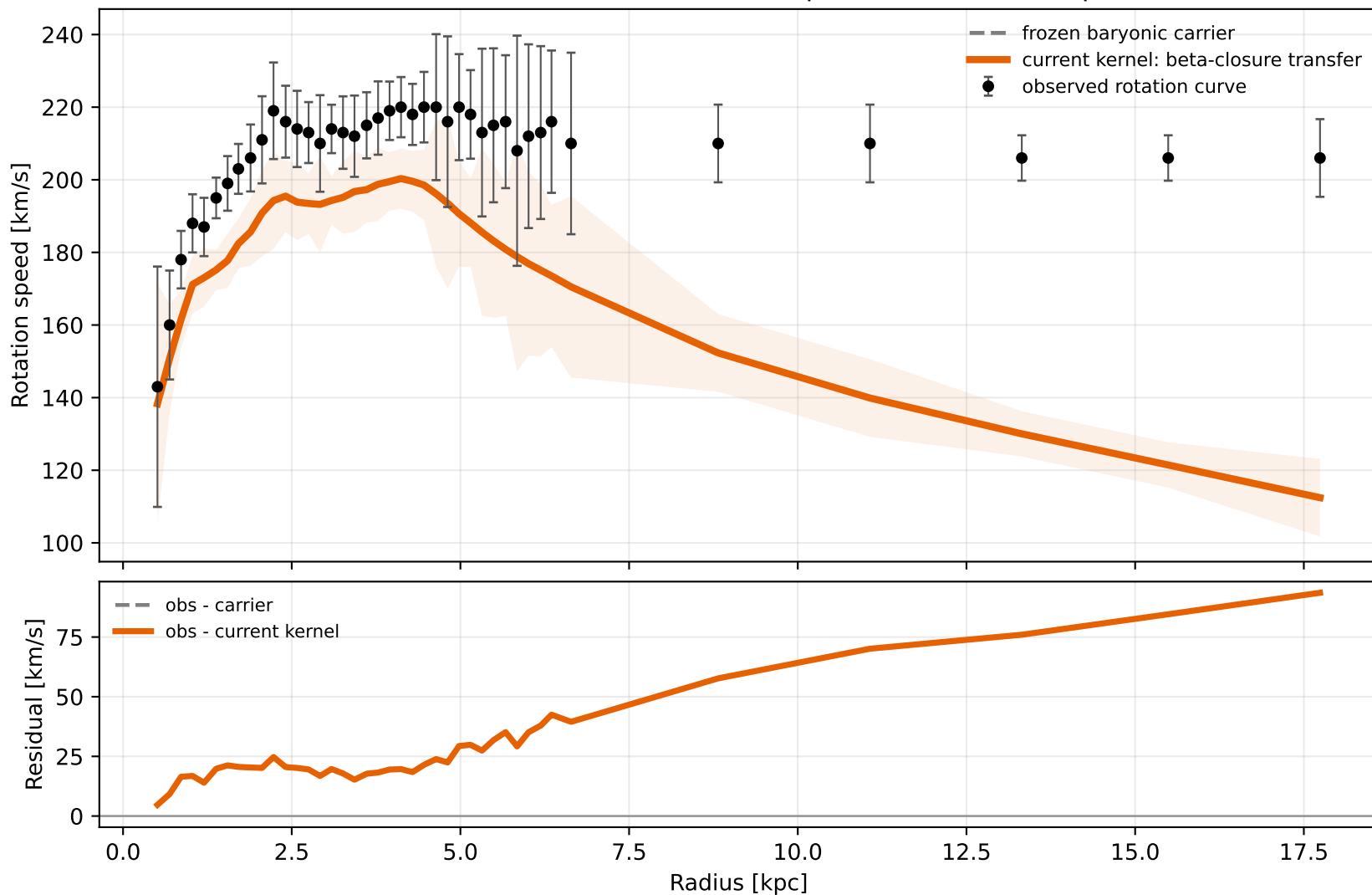
NGC3521: beta-closure transfer control comparison (does not improve carrier)
