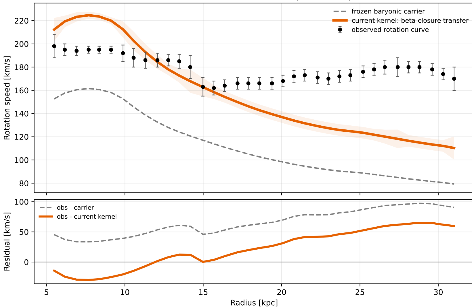
NGC4013: beta-closure transfer control comparison (improves carrier)
