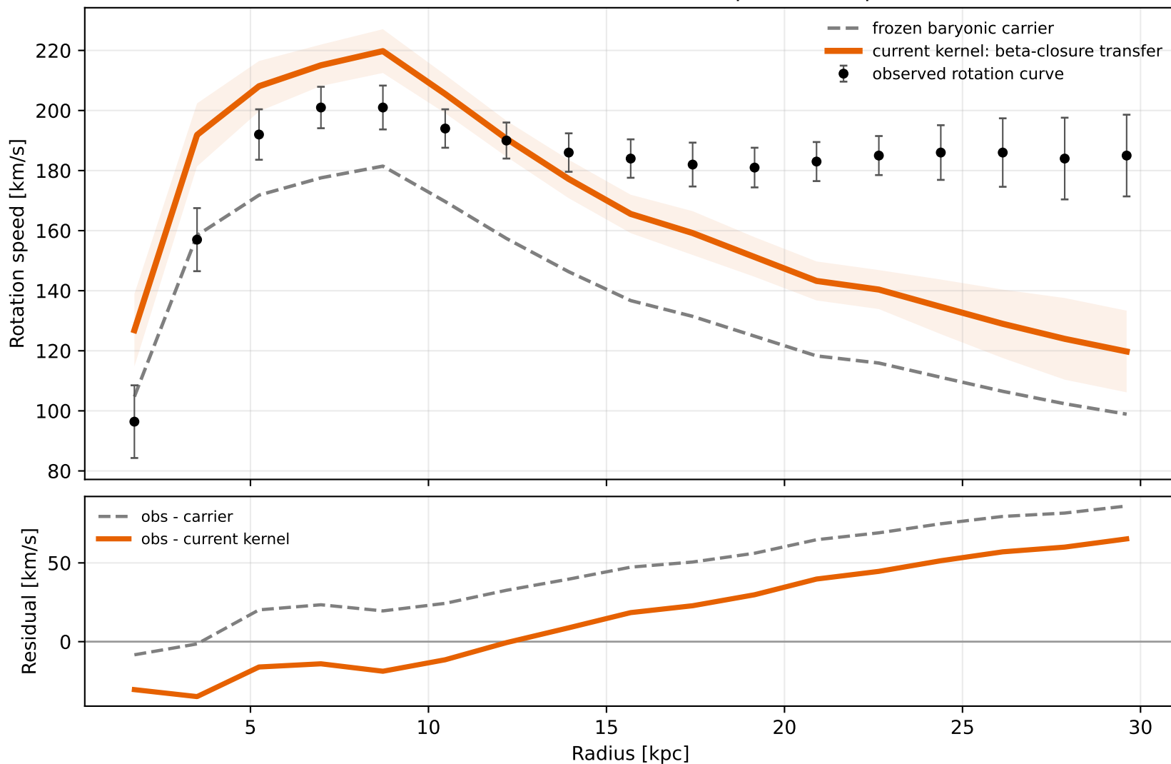
NGC4157: beta-closure transfer control comparison (improves carrier)
