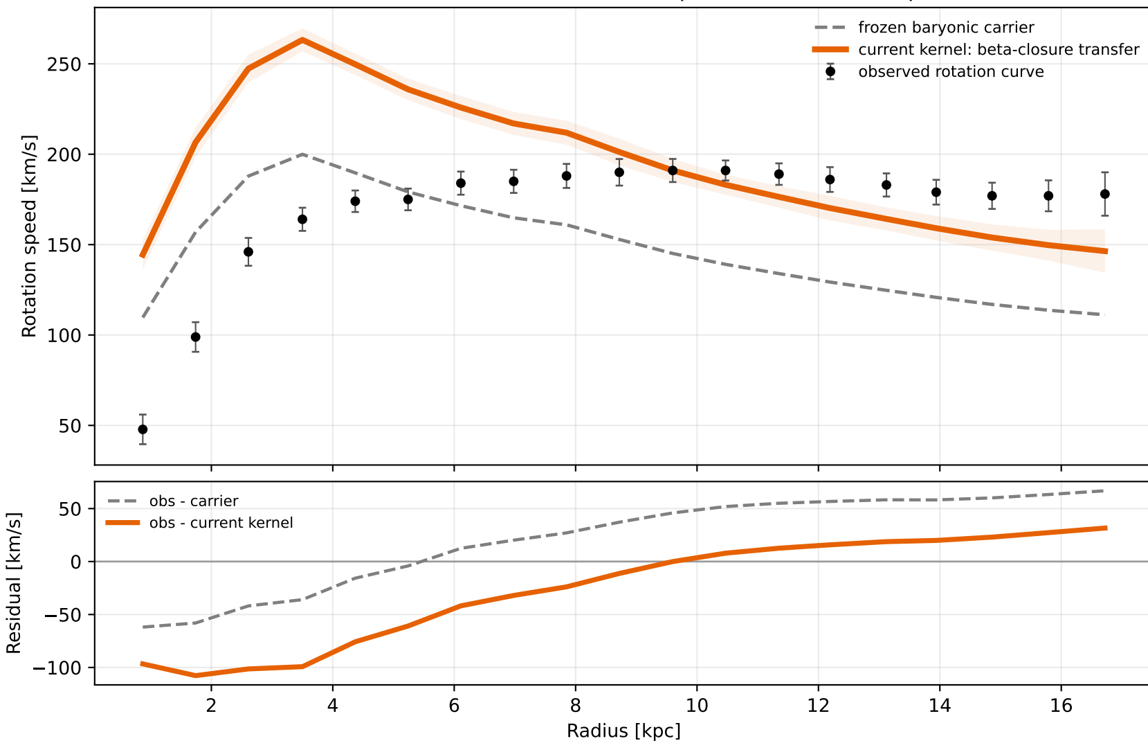
NGC4217: beta-closure transfer control comparison (does not improve carrier)
