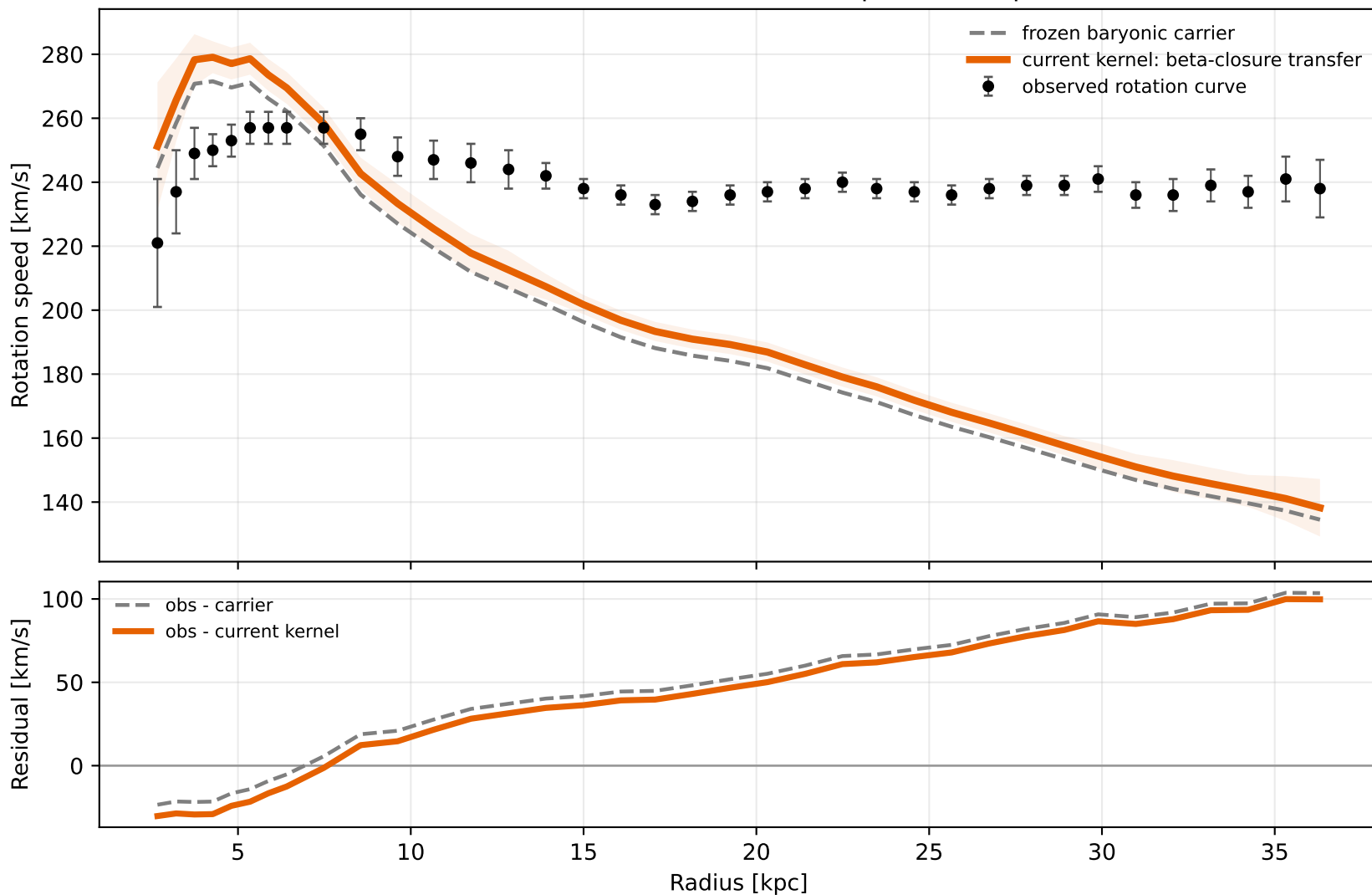
NGC7331: beta-closure transfer control comparison (improves carrier)
