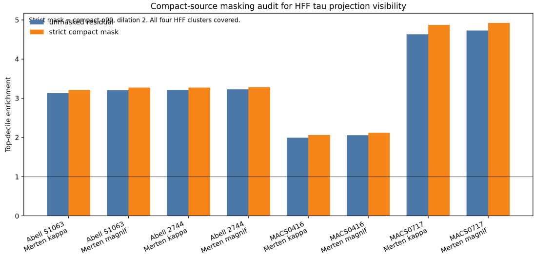
Figure 5: Compact-source masking audit. Bars compare unmasked and strict compact-masked X-ray/lensing enrichment for the covered clusters. The test does not prove a physical mechanism, but it argues against the simplest compact X-ray-peak contamination explanation for the enrichment statistic.
