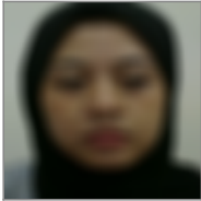
neutral
