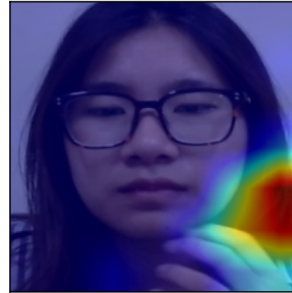
Early concat
