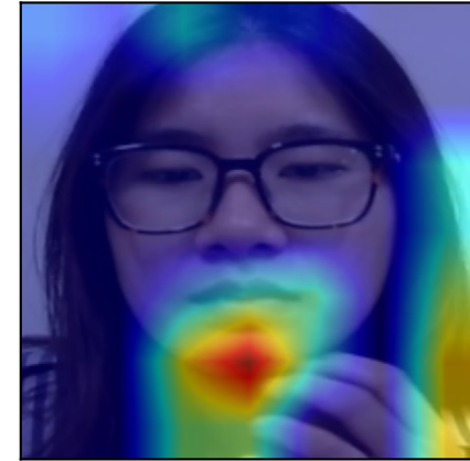
Early gated
