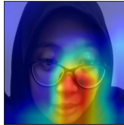
Early concat
