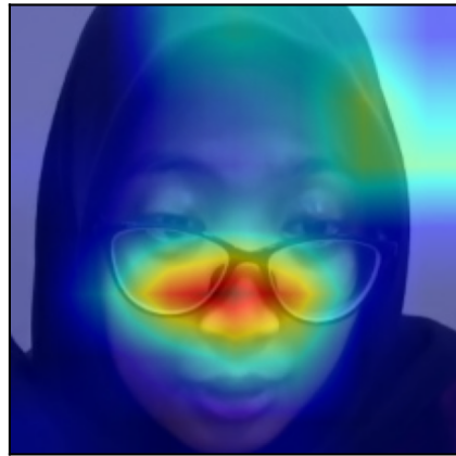
CNN_TL (unimodal)
