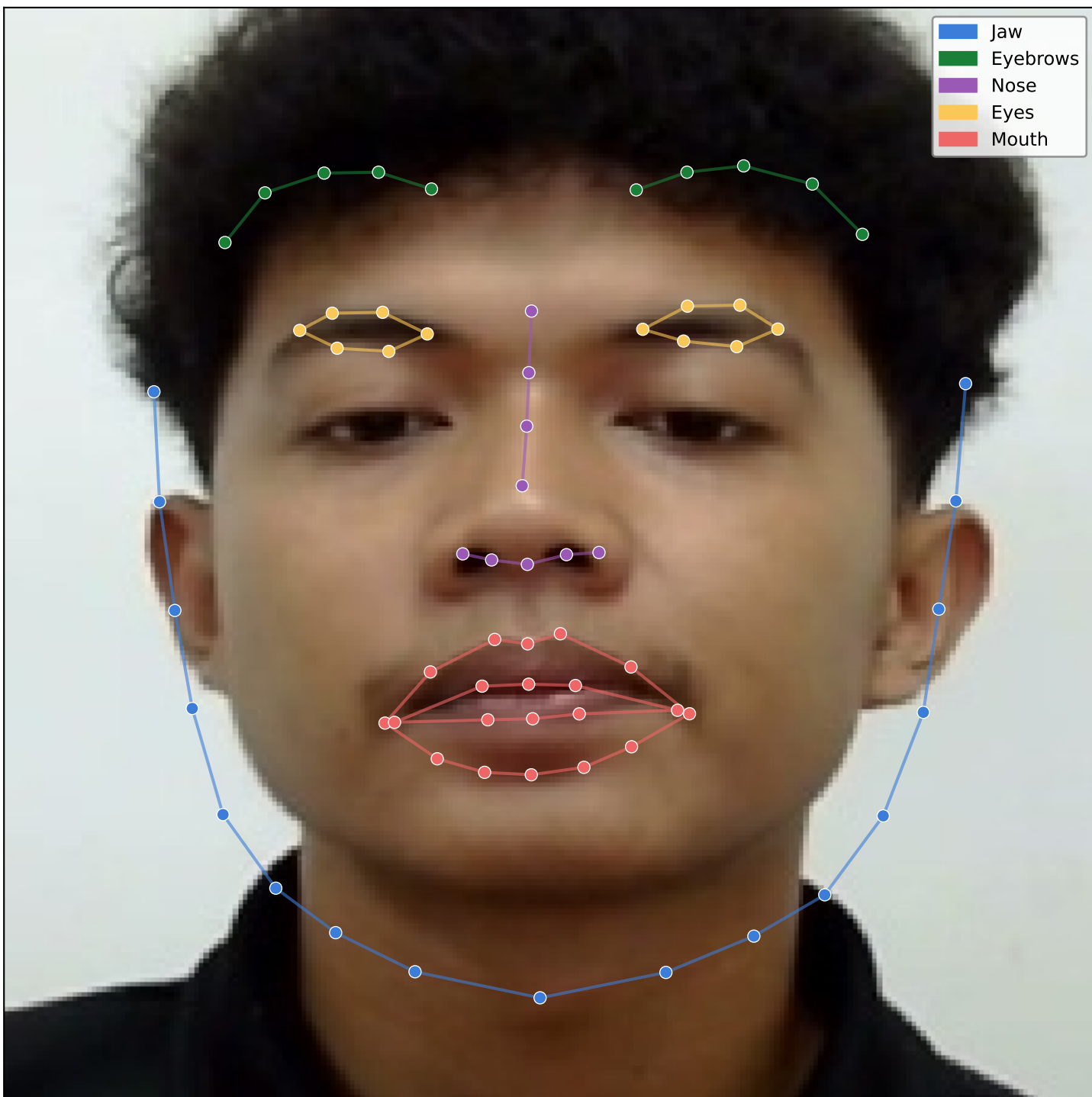
68-point Facial Landmark — Color-coded by Anatomical Region
