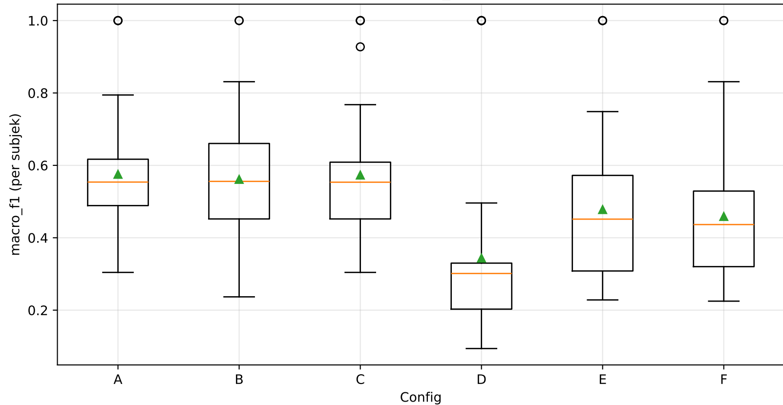
LOSO — distribusi macro_f1 antar 37 subjek
