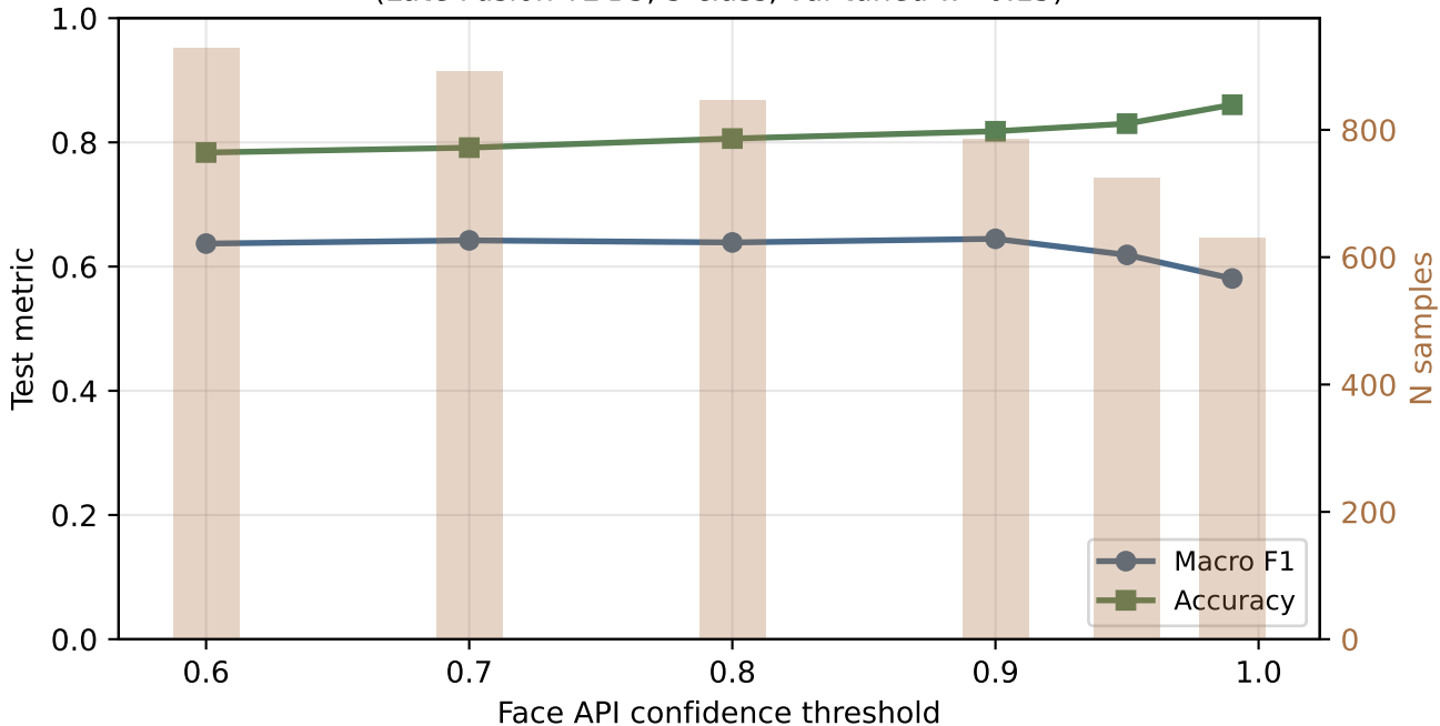
Test Performance vs Face API Confidence Threshold (Late Fusion TL B3, 3-class, val-tuned w=0.15 )
