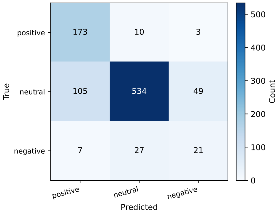
3-Class CM — Late Fusion TL B3
